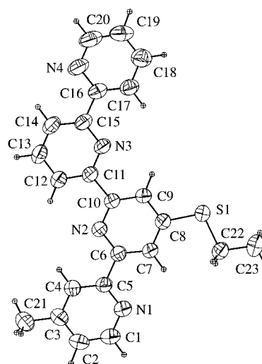
Figure 10. Proton NMR shifts of H-3' and H-5' in dicopper(I)-qtpy helicates: (A) 4',4''-bis(methylthio)-qtpy 19 ; (B) [\text{Cu}_2(\mathbf{1a})_2][\text{PF}_6]_2 ; (C) [\text{Cu}_2(\mathbf{1b})_2][\text{PF}_6]_2 ; (D) [\text{Cu}_2(\mathbf{1c})_2][\text{PF}_6]_2 ; (E) [\text{Cu}_2(\mathbf{1d})_2][\text{PF}_6]_2 . Shifts of the HH and HT isomers from the same positions are connected by a line.
