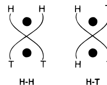
Figure 1. Head-to-head and head-to-tail isomers of a dinuclear double helicate.
