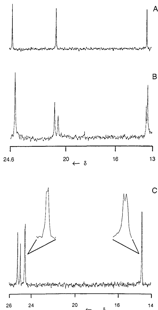
Figure 8. Partial ^{13}\text{C} NMR spectra (75 MHz): (A) ligand 1b in 70% (\text{CD}_3)_2\text{SO} –30% \text{CDCl}_3 ; (B) [\text{Cu}_2(\mathbf{1b})_2][\text{PF}_6]_2 in (\text{CD}_3)_2\text{SO} ; (C) [\text{Cu}_2(\mathbf{1e})_2][\text{PF}_6]_2 in (\text{CD}_3)_2\text{SO} .
