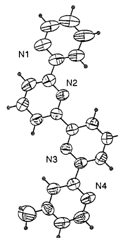
Figure 4. Solid state structure of 4-methyl-2,6':2'',6'''-quaterpyridine ( 1h ).
