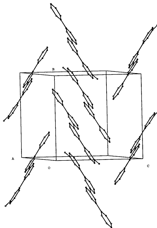
Figure 6. Packing of 4-methyl-2,6':2',6'':2'',6'''-quaterpyridine ( 1h ) in the crystal lattice.
